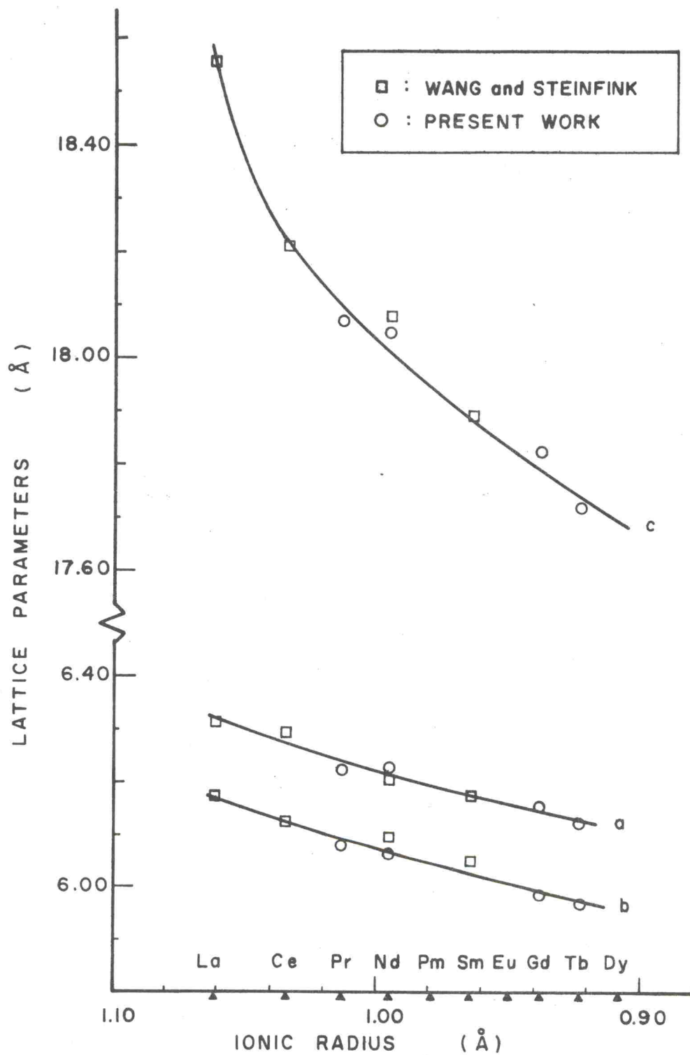
Fig. 19.--Variation of Lattice Parameters With Ionic Radius of \text{LaSb}_2 Type Rare Earth Diantimonides.
